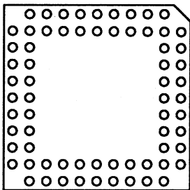
FIGURE 8 — HOLE SIDE of NOTCHED 68-PIN SOCKET
